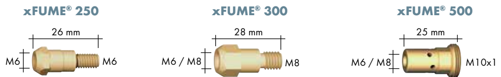
Contact tip holder (10 pcs.)
